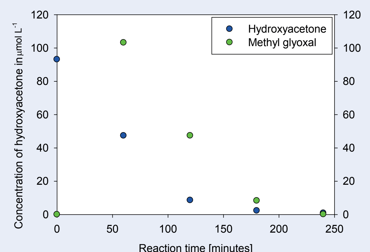
Figure 5: Oxidation of hydroxyacetone.
