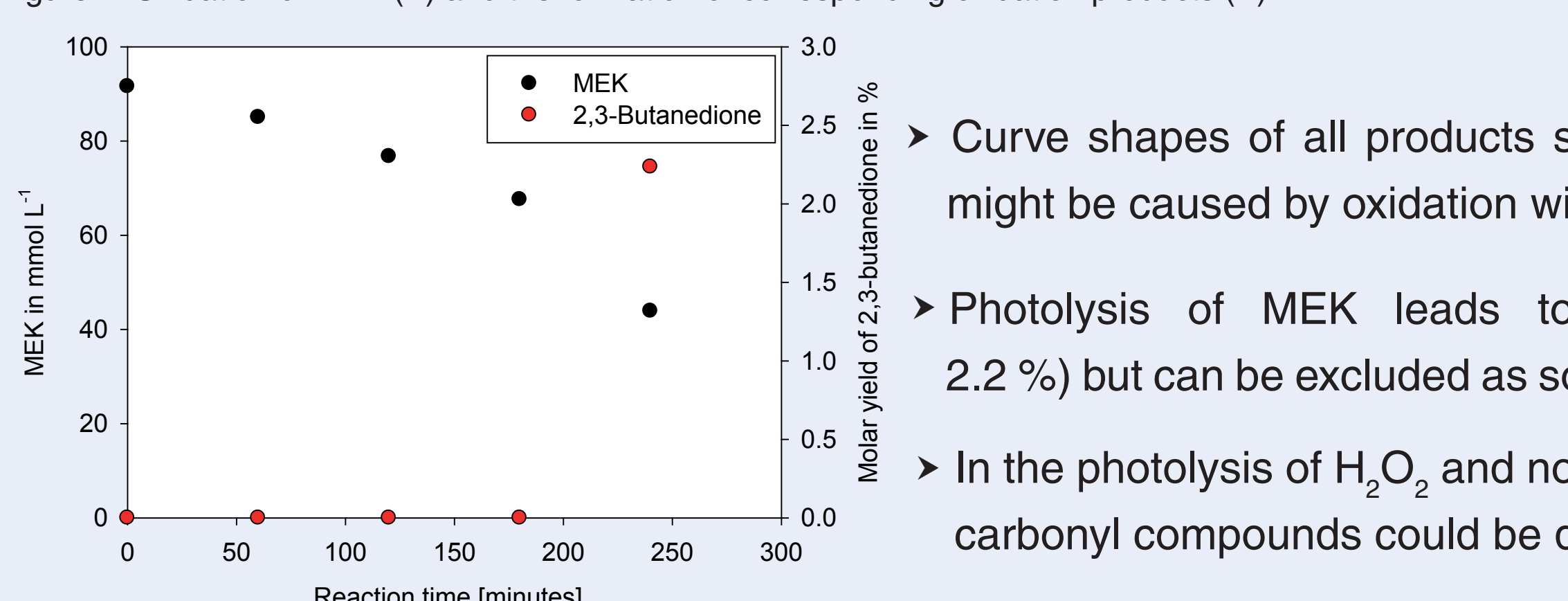
Figure 3: Photolysis of MEK and formation of 2,3-butanedione.
